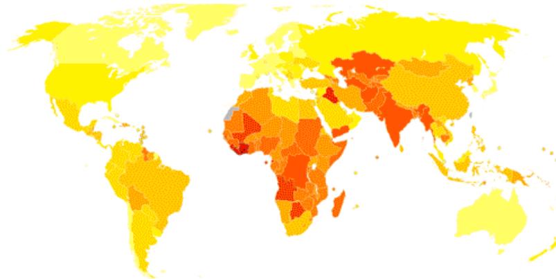
Prematurity and low birth weight world map
